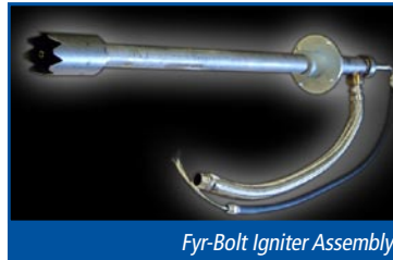
Fyr-Bolt Igniter for a T-fired Boiler
